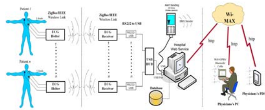
Fig.6:: The structure of the signal processing system in the ECG monitoring.
